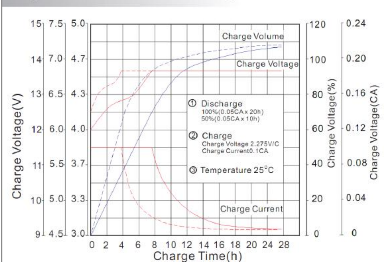
Charge characteristic Curve for standby use
